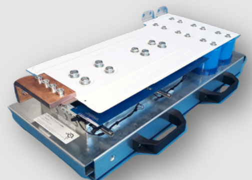
ZOPF Pro 2.5 MW - Water
